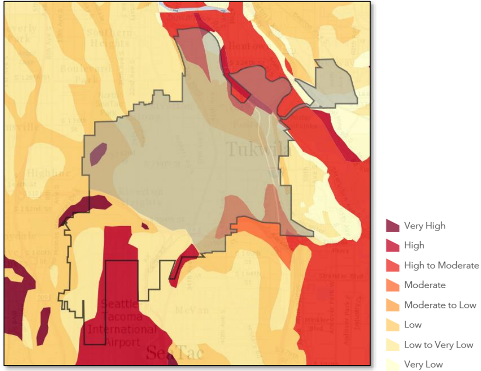
Figure 1: liquefaction potential in and around KCWD 125
