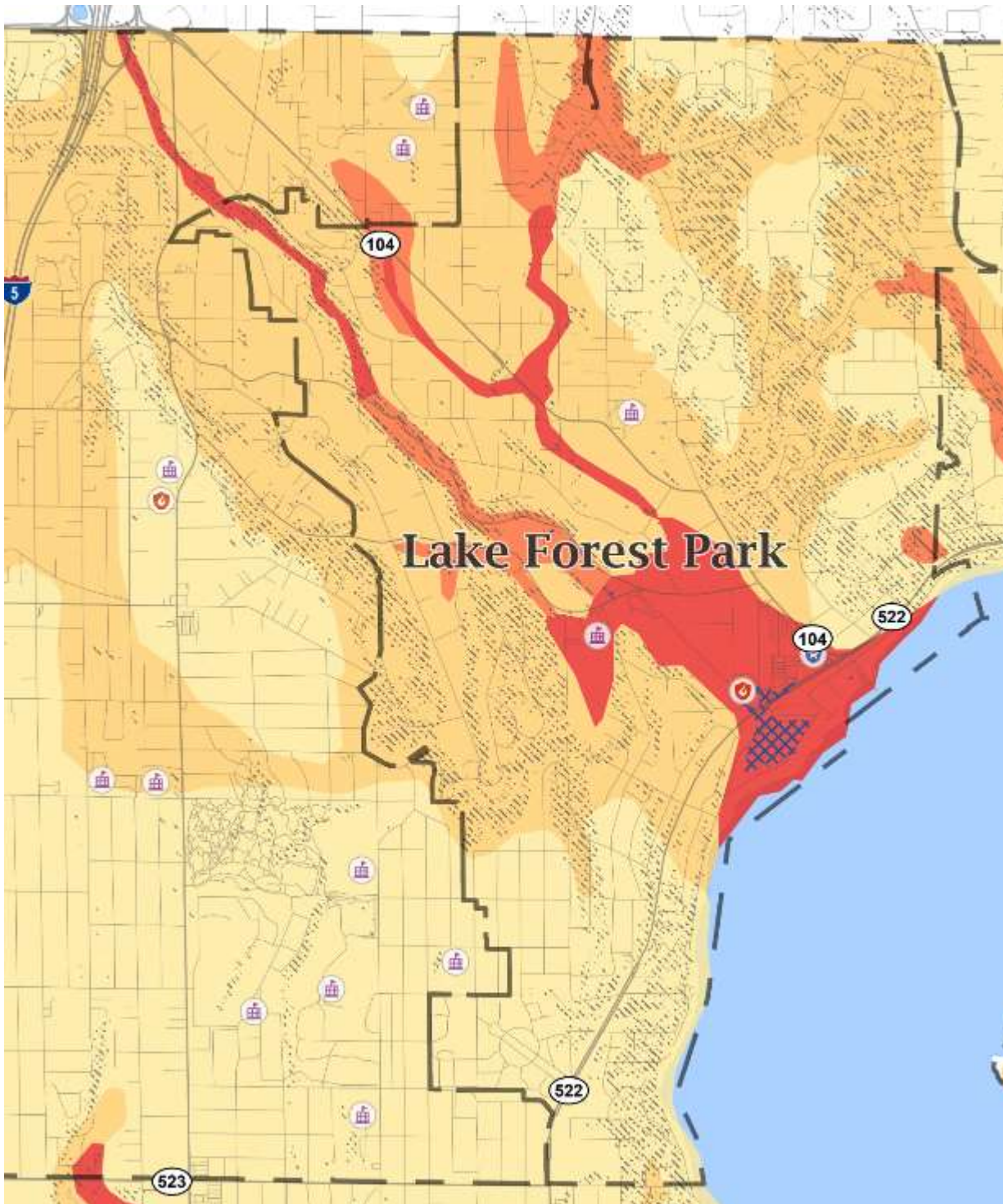
Figure 1: Liquefaction Zones
