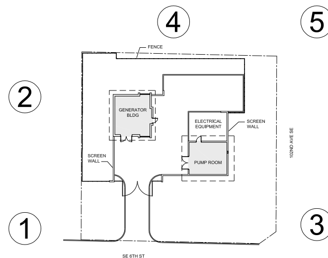
Grade Level Plan - Existing
