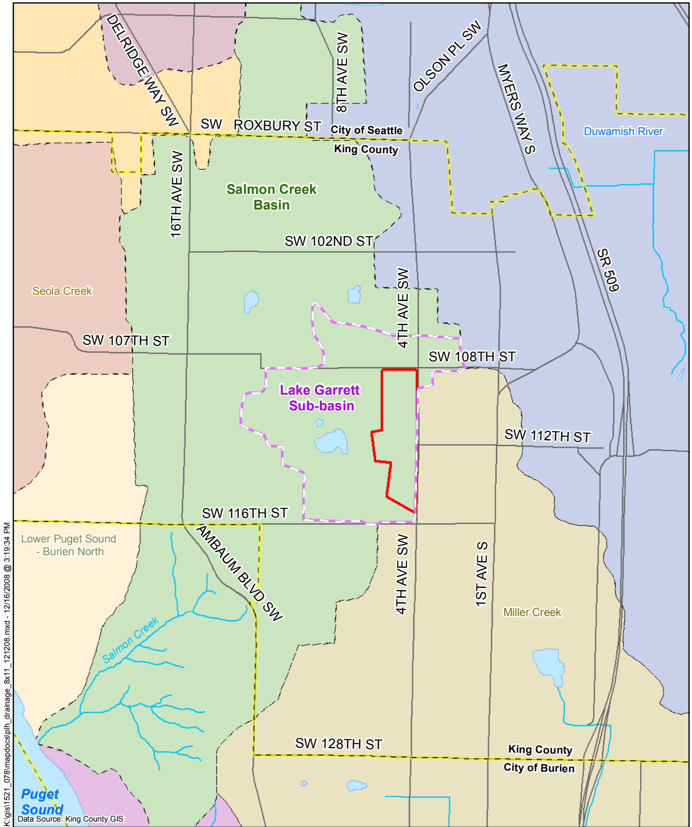
Figure 3.16-1 Drainage Sub-basins
