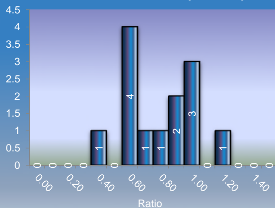
2016 Ratio Frequency
