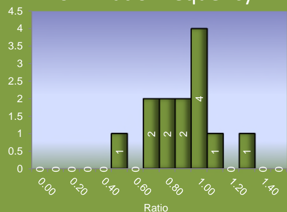
2017 Ratio Frequency
